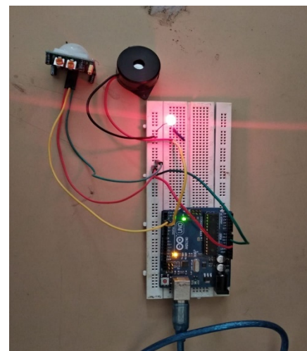
Fig.6. Circuit for human presence detection with PIR sensor
