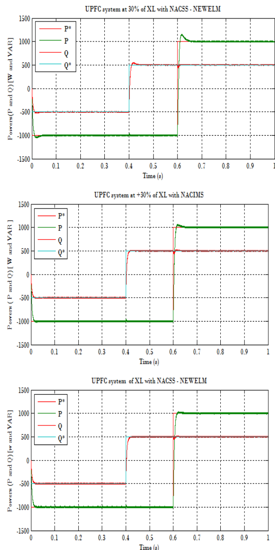
Fig. 19. Powers (P and Q) of the control system with (NACSS-NEWELM) at \pm 30\% of XL
