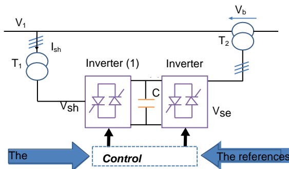
Fig.1. Basic circuit configuration of a UPFC.
