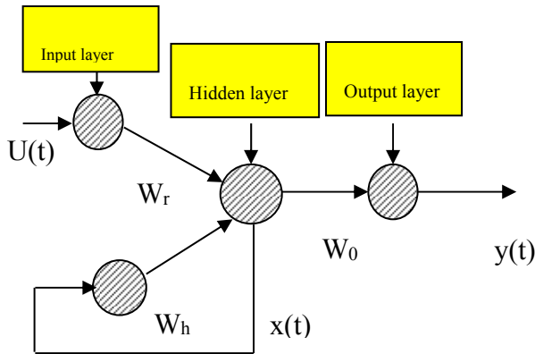
Fig. 12. Structure of the NEWELM
