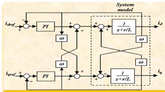
Fig.3. Control design with PI corrector.
