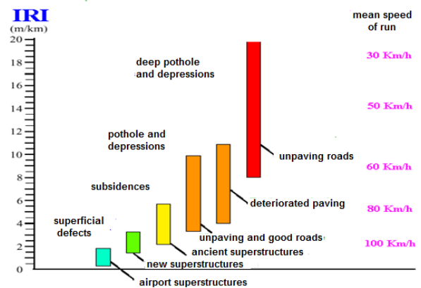
Fig. 24 – Roughness index
