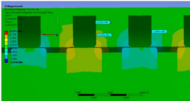
Fig. 11 – Particular of the directional magnetic flux density (intermediate position); flux values are highlighted.
