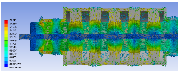
Fig. 7: Magnetic field flux lines (maximum concatenated flux position).
