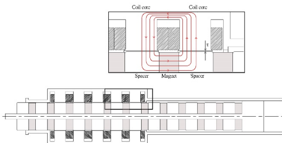
Fig. 2: Damper with the stem in the maximum concatenated flux position.
