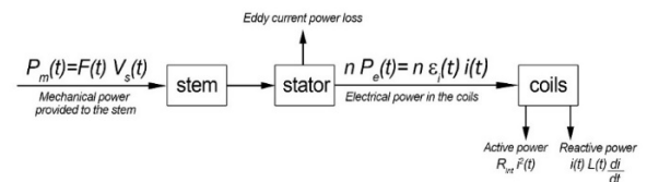
Fig. 14: Block diagram of the energy balance.
