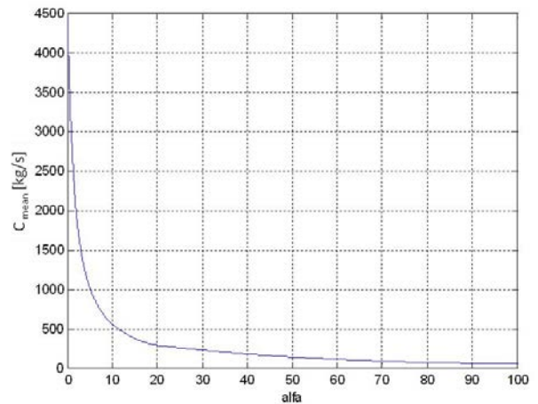
Fig. 21: Mean damping coefficient versus \alpha ratio.
