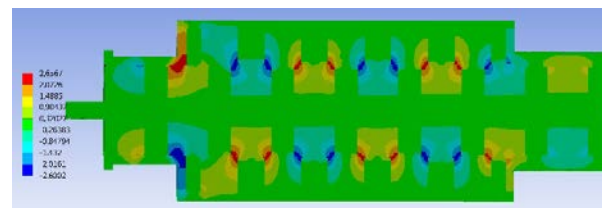
Fig. 10: Directional magnetic flux density (minimum concatenated flux position).
