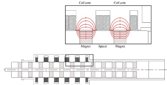
Fig. 3: Damper with the stem in the position of minimum concatenated flux.
