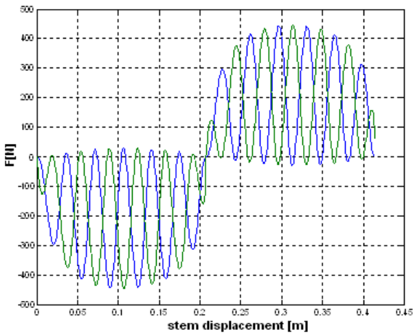
Fig. 18: Force generated by the two blocks of coils versus the stem position.
