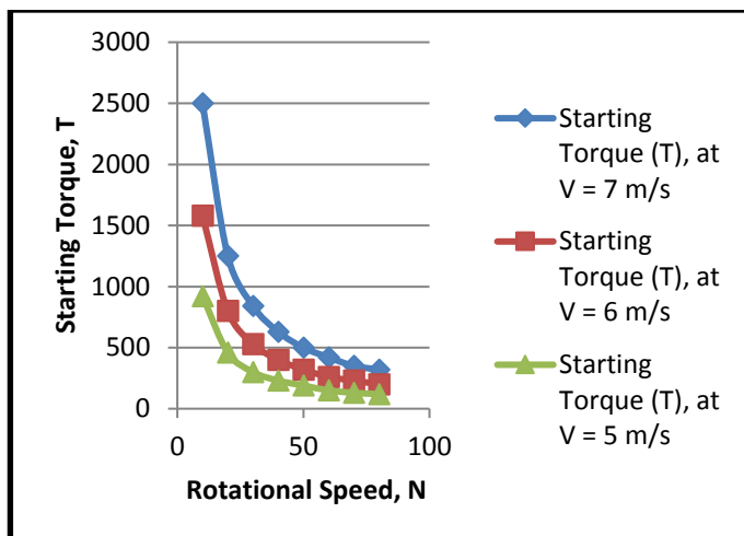
Fig.5 Effect of changing wind speed on starting torque
