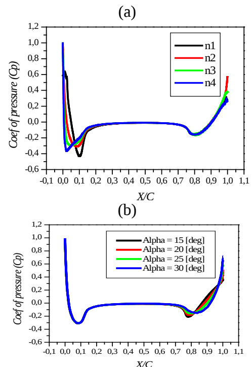
Fig.10: C_p distribution around the UV for n (a) and \alpha (b)
