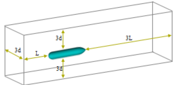
Fig.2: Computational domain
