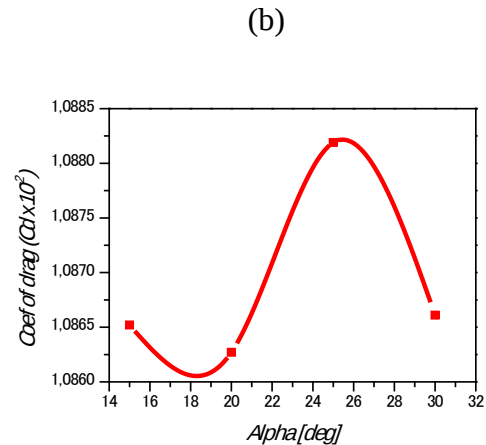
Fig.9: Drag coefficients of different value of n (Fig (a)) and the angle \alpha (Fig (b))
