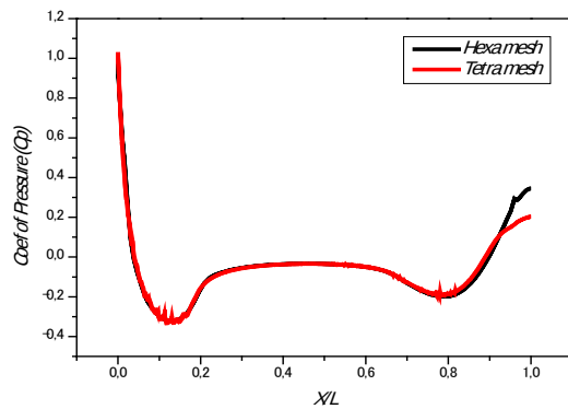
Fig.4: Pressure coefficient comparison for tetra and hexa meshes
