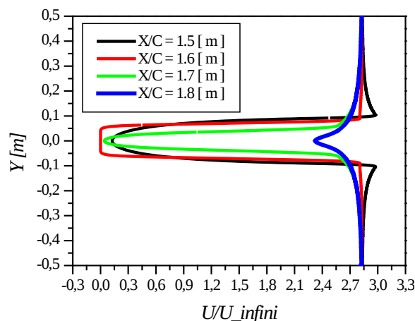
Fig.11: Velocity profile in XY plane
