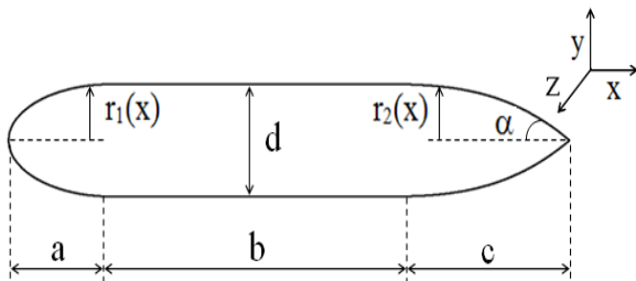
Fig.1: AUV parameters of Myring Equation
