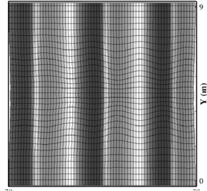
Figure 4 Detailed plane view of the instantaneous wave field obtained with the highly distorted curvilinear computational grid. Only one coordinate line out of every two is shown.
