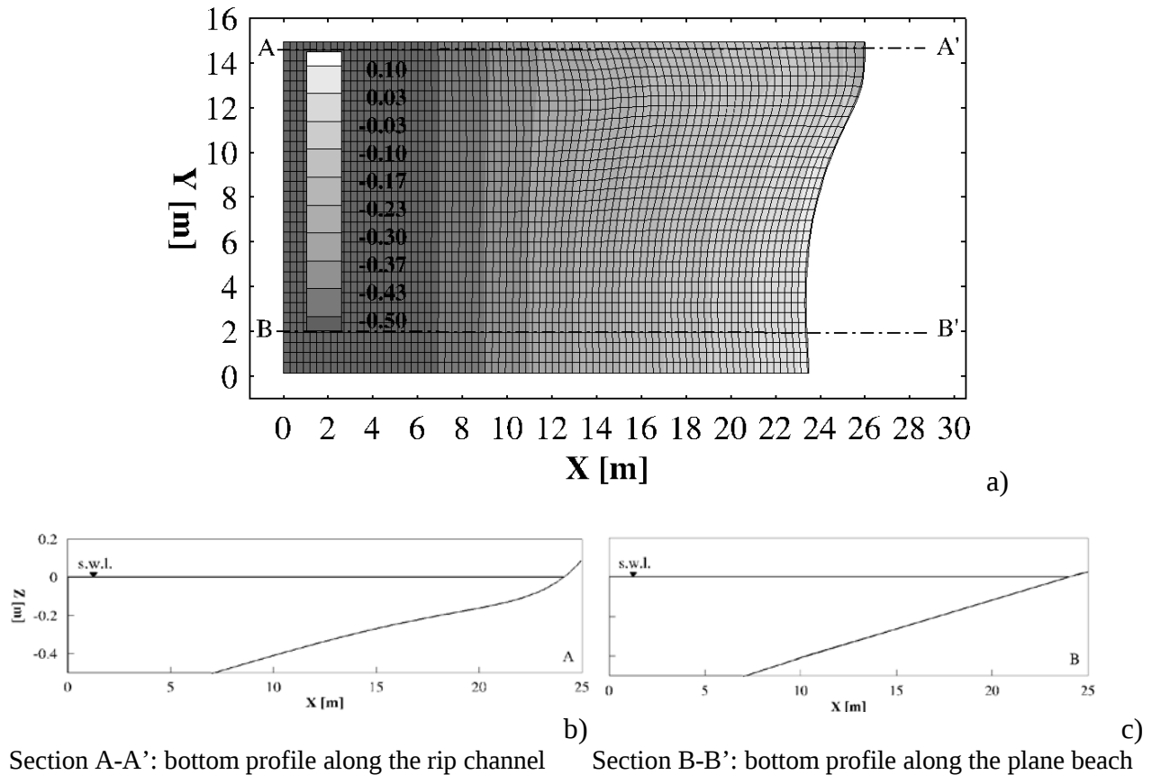
Figure 6 Bathymetry (Only one out of every five coordinate lines is shown). (b-c): bottom profiles in section A-A' and B-B'.
