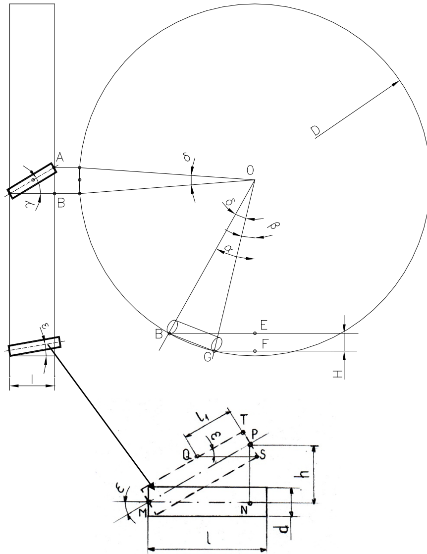
Fig.4: Calculation of the volume of water extracted from the river by a collector tube.
