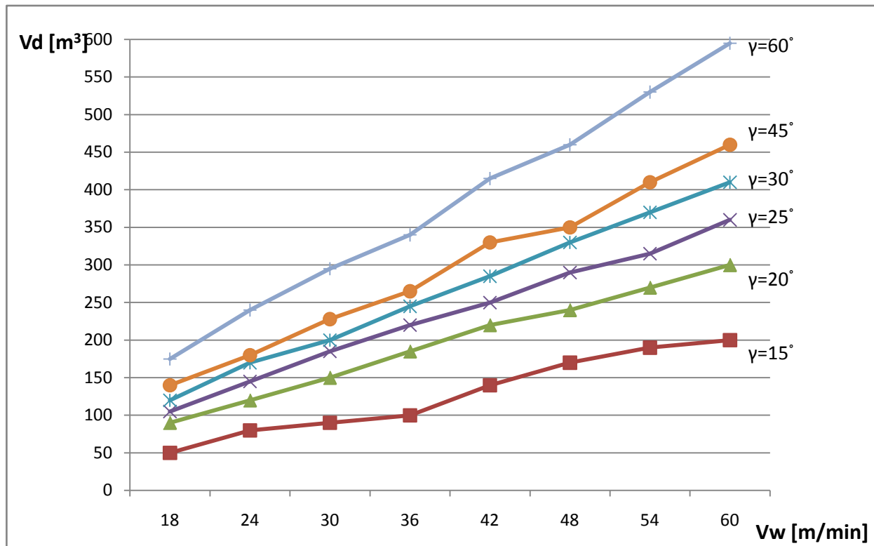
Fig.5: Dependence of the volume of water extracted from the river in a day (Vd), depending on the angle of installation of the collecting tubes on the circumference of the rotor (angle \gamma ) and the speed of the water of the river (Vw).
