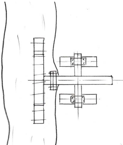
Fig.7: Mounting the installation directly on the river bank.
