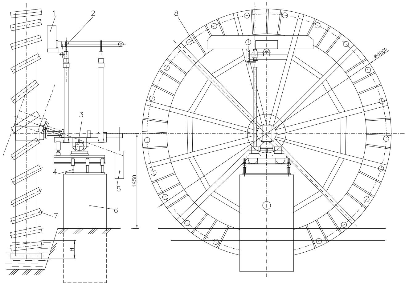
Fig.3: Sketch of an undershot water wheel used for irrigation of dry lands.
