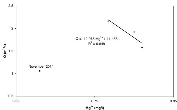
Fig. 13, Relationship between the Mg 2+ concentration and Pertuso Spring discharge values obtained with the combined Magnesium-discharge tracer approach
