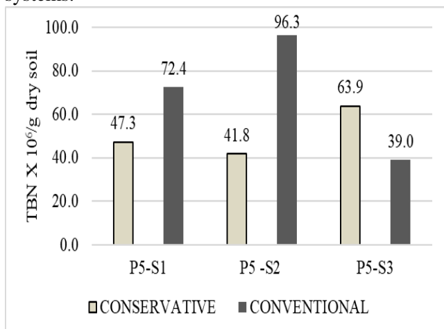
Fig. 1. The size of the edaphic bacterial communities under the two soil tillage systems - autumn 2016
