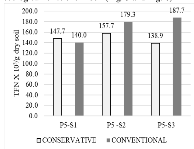
Fig. 3. The size of the edaphic microfungi communities under the two soil tillage systems - autumn 2016
