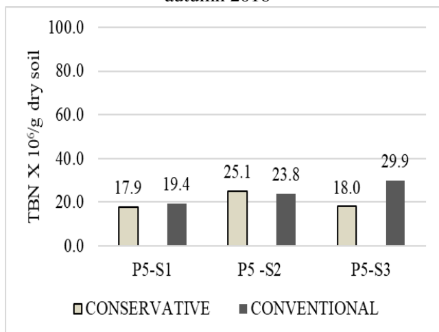
Fig. 2. The size of the edaphic bacterial communities under the two soil tillage systems - spring 2017
