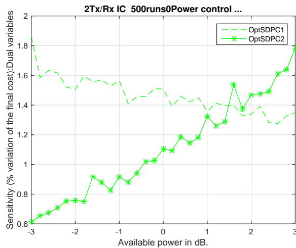
Figure 4: K= 2 BS with M= 2 antennas and the regulation mask is \rho = 0 dB. Sensitivity analysis of the constraints in P_2 (i.e. OptSDPC1 for constraint P_{2-a} : p_q^* ||\mathbf{b}_q|| \leq P_{max} and OptSDPC2 for constraint P_{2-b} : p_q^* a_{qI} \leq \alpha\rho ).
