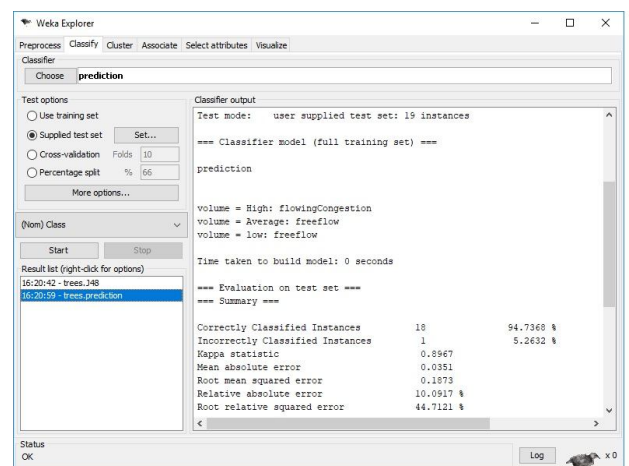
Figure 4:Prediction of traffic congestion
