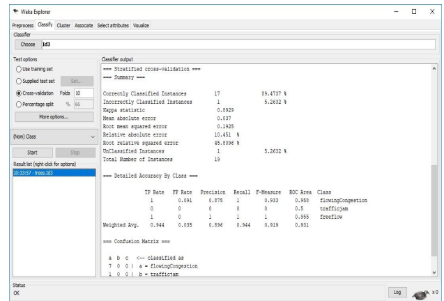
Figure 3: Classified Data
