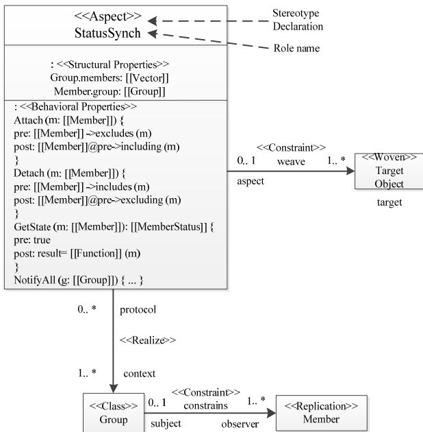
Figure 2. Fault-tolerant aspect modeling method based on copy mechanism
