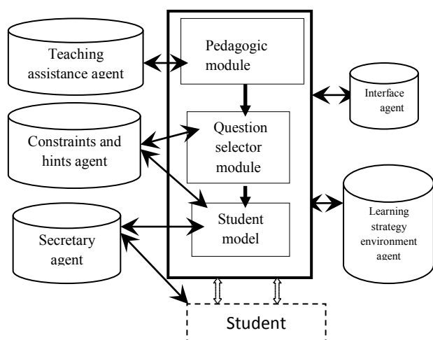
Fig. (4) Types of Agents in the AG_TUTOR
