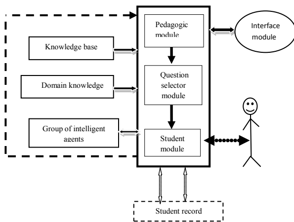
Fig. (2) The structure of AG_TUTOR
